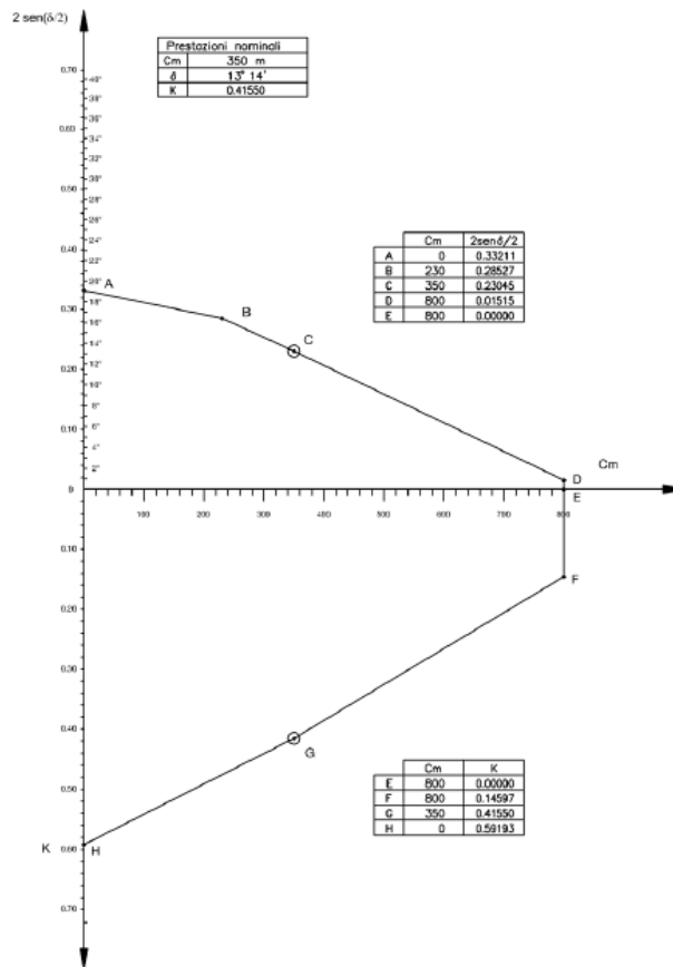
Fig E4 – Example of Italian Standard M Type Lattice Tower DT Full Load - Utilization Diagram
