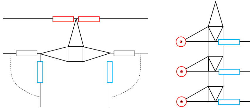
Connection scheme for a derivation tower.
